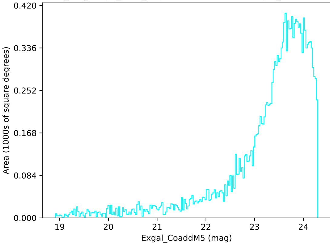
mw_roll_bulge_v3.3_10yrs Yr 3-4 u band: Exgal_CoaddM5
