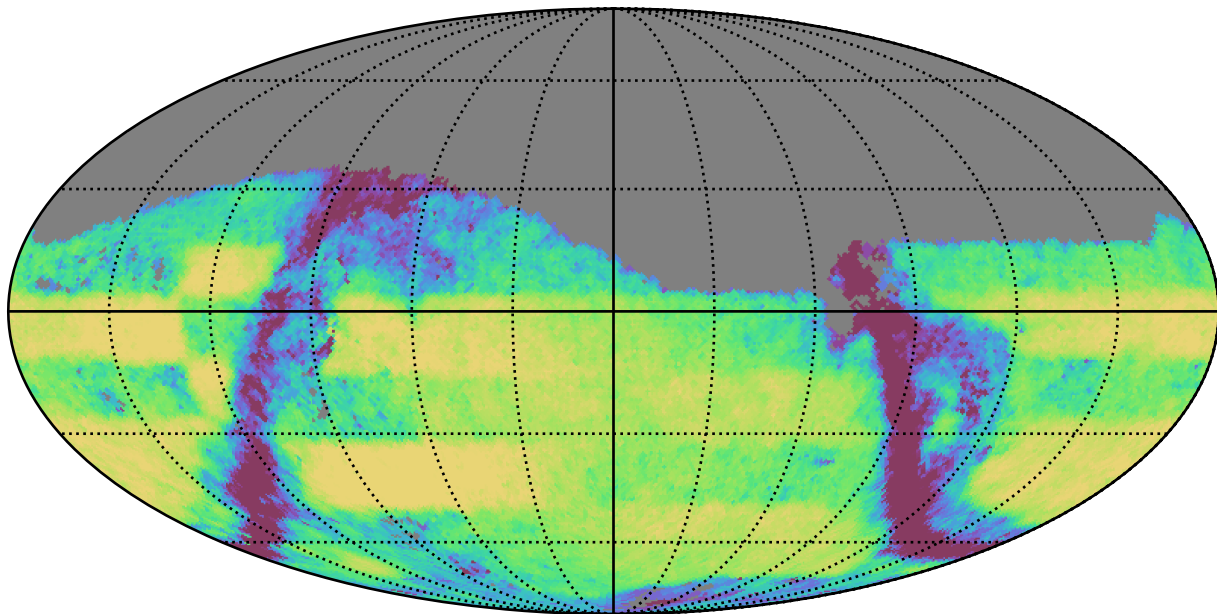
mw_roll_bulge_v3.3_10yrs Yr 3-4 r band: Exgal_CoaddM5
