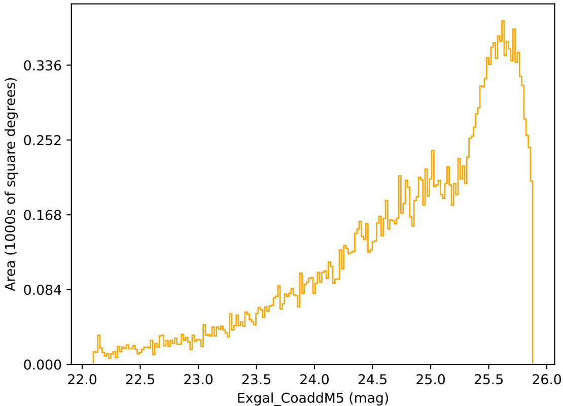
mw_roll_bulge_v3.3_10yrs Yr 3-4 r band: Exgal_CoaddM5
