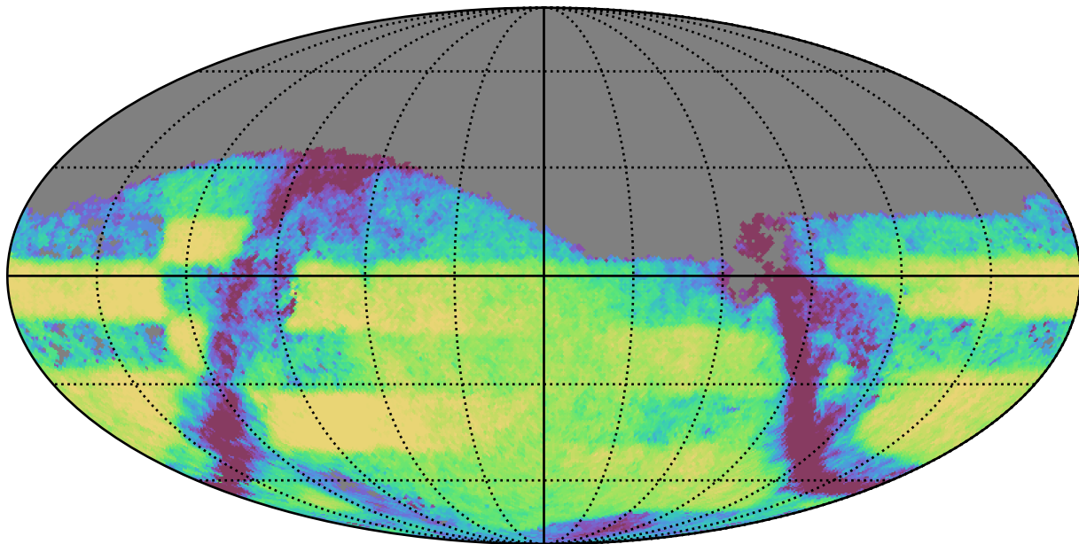
mw_roll_bulge_v3.3_10yrs Yr 3-4 i band: Exgal_CoaddM5
