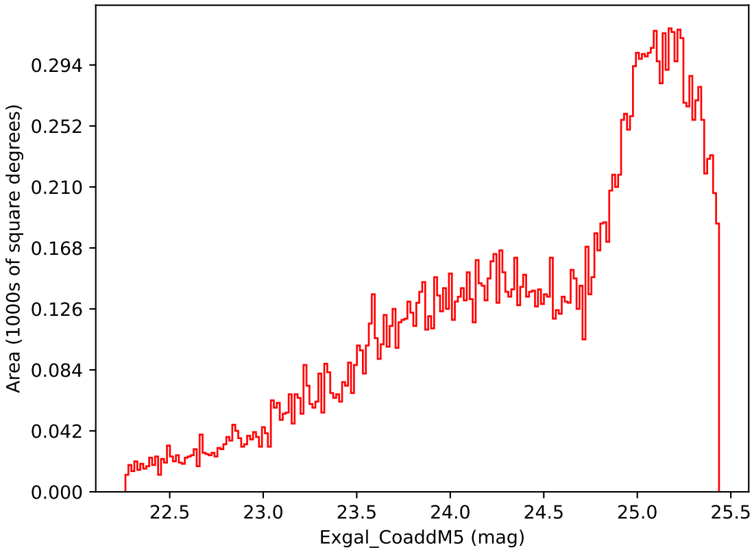
mw_roll_bulge_v3.3_10yrs Yr 3-4 i band: Exgal_CoaddM5
