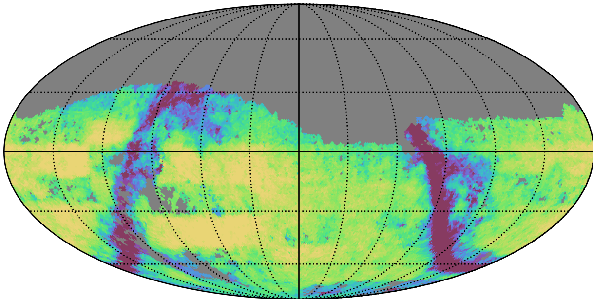
mw_roll_bulge_v3.3_10yrs Yr 3-4 g band: Exgal_CoaddM5
