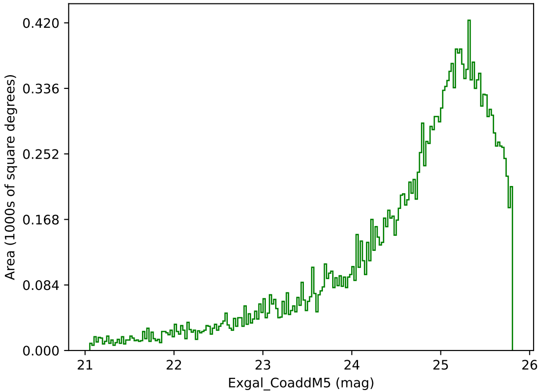
mw_roll_bulge_v3.3_10yrs Yr 3-4 g band: Exgal_CoaddM5
