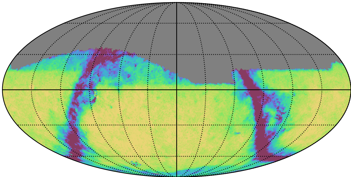
mw_roll_bulge_v3.3_10yrs Yr 1 r band: Exgal_CoaddM5
