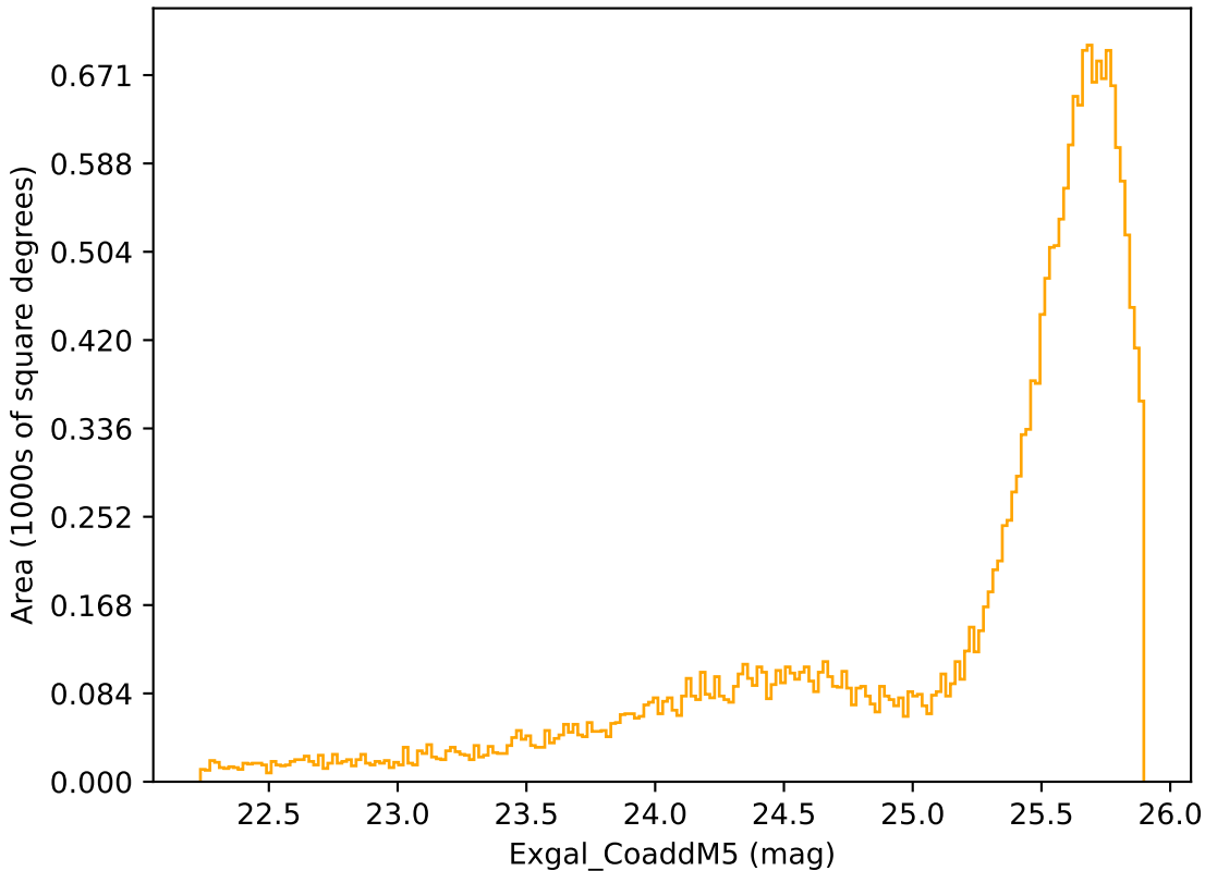
mw_roll_bulge_v3.3_10yrs Yr 1 r band: Exgal_CoaddM5
