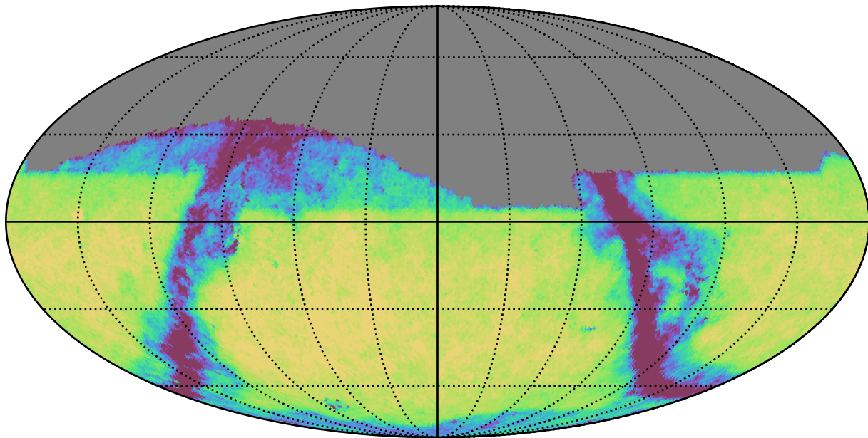
mw_roll_bulge_v3.3_10yrs Yr 1 i band: Exgal_CoaddM5
