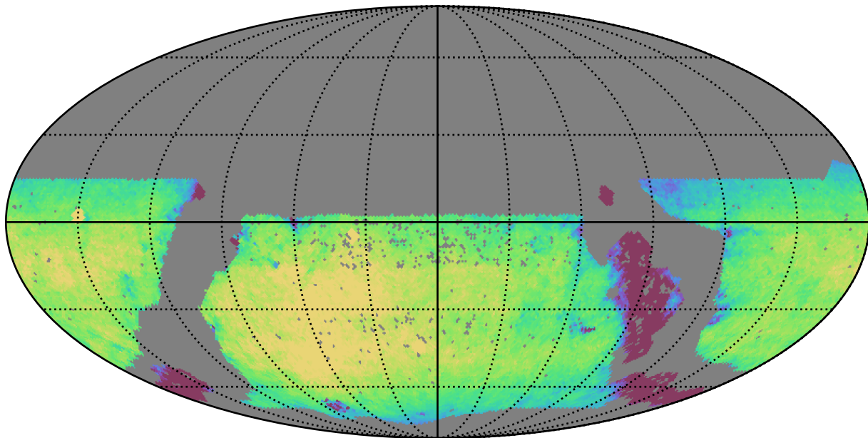
mw_roll_bulge_v3.3_10yrs WFD z band: Exgal_CoaddM5
