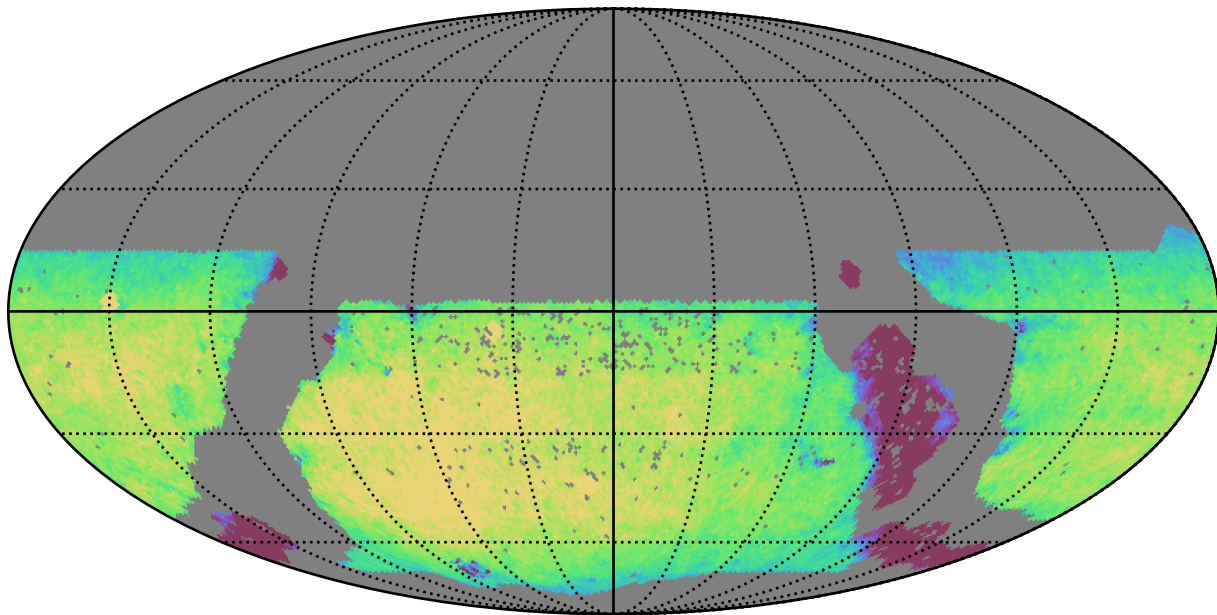
mw_roll_bulge_v3.3_10yrs WFD y band: Exgal_CoaddM5
