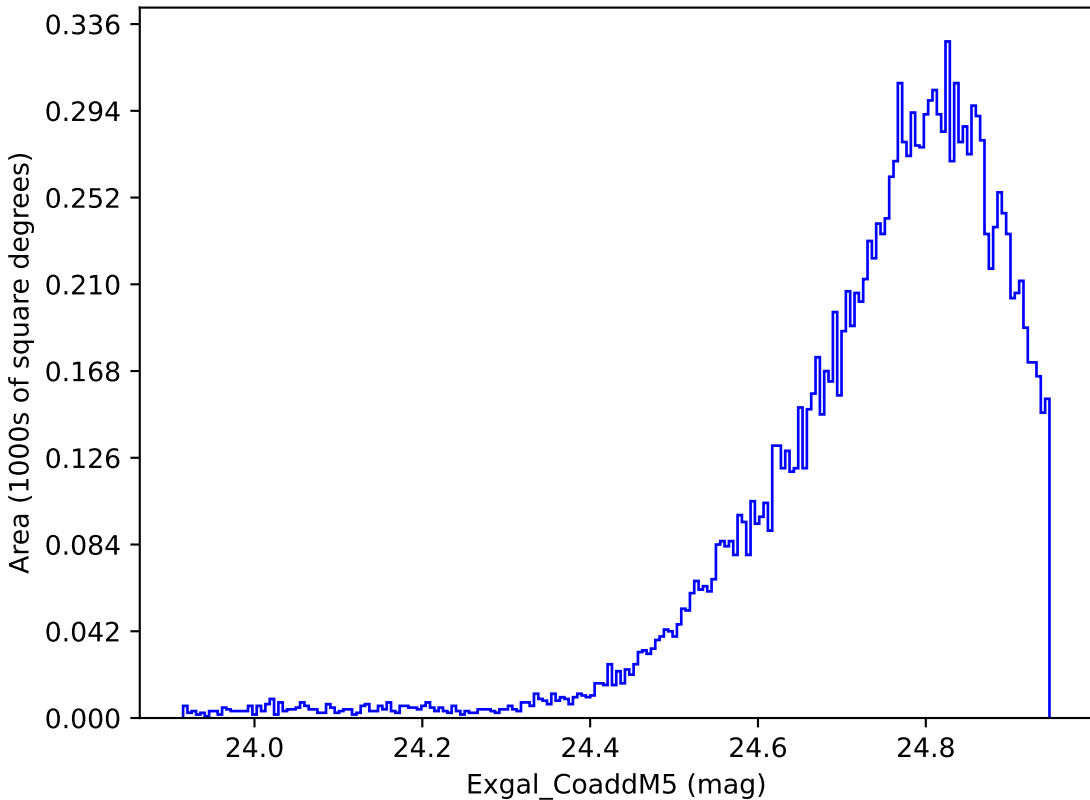
mw_roll_bulge_v3.3_10yrs WFD y band: Exgal_CoaddM5
