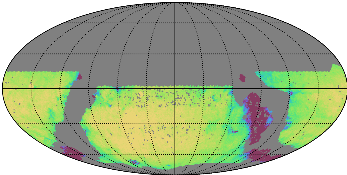
mw_roll_bulge_v3.3_10yrs WFD u band: Exgal_CoaddM5
