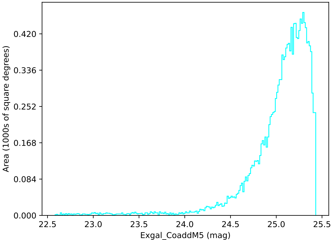
mw_roll_bulge_v3.3_10yrs WFD u band: Exgal_CoaddM5
