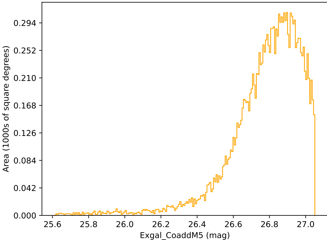
mw_roll_bulge_v3.3_10yrs WFD r band: Exgal_CoaddM5
