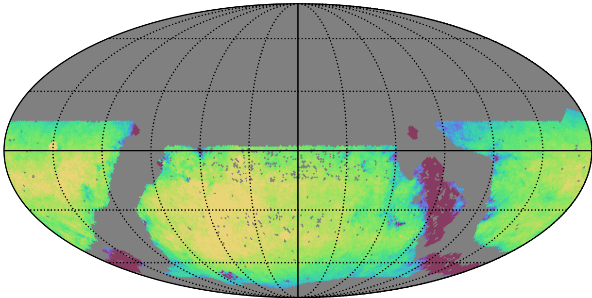
mw_roll_bulge_v3.3_10yrs WFD i band: Exgal_CoaddM5
