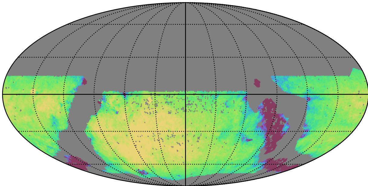
mw_roll_bulge_v3.3_10yrs WFD g band: Exgal_CoaddM5
