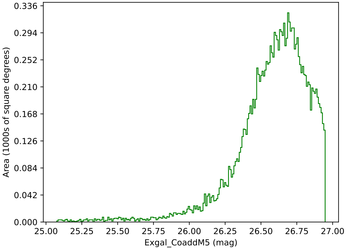
mw_roll_bulge_v3.3_10yrs WFD g band: Exgal_CoaddM5
