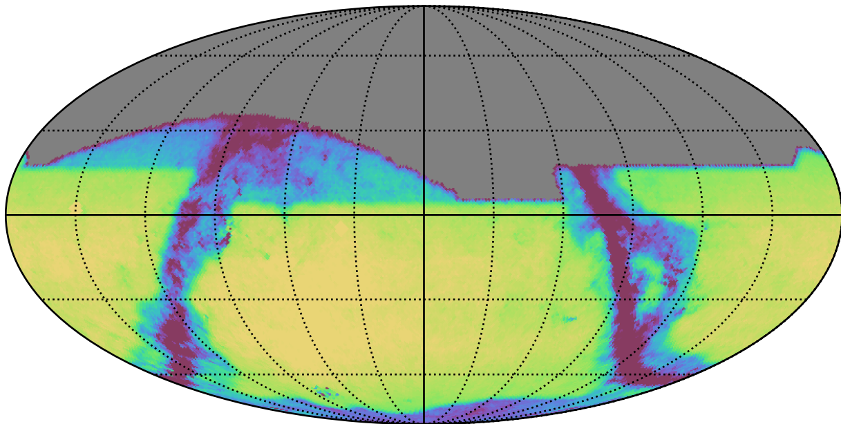
mw_roll_bulge_v3.3_10yrs All sky z band: Exgal_CoaddM5
