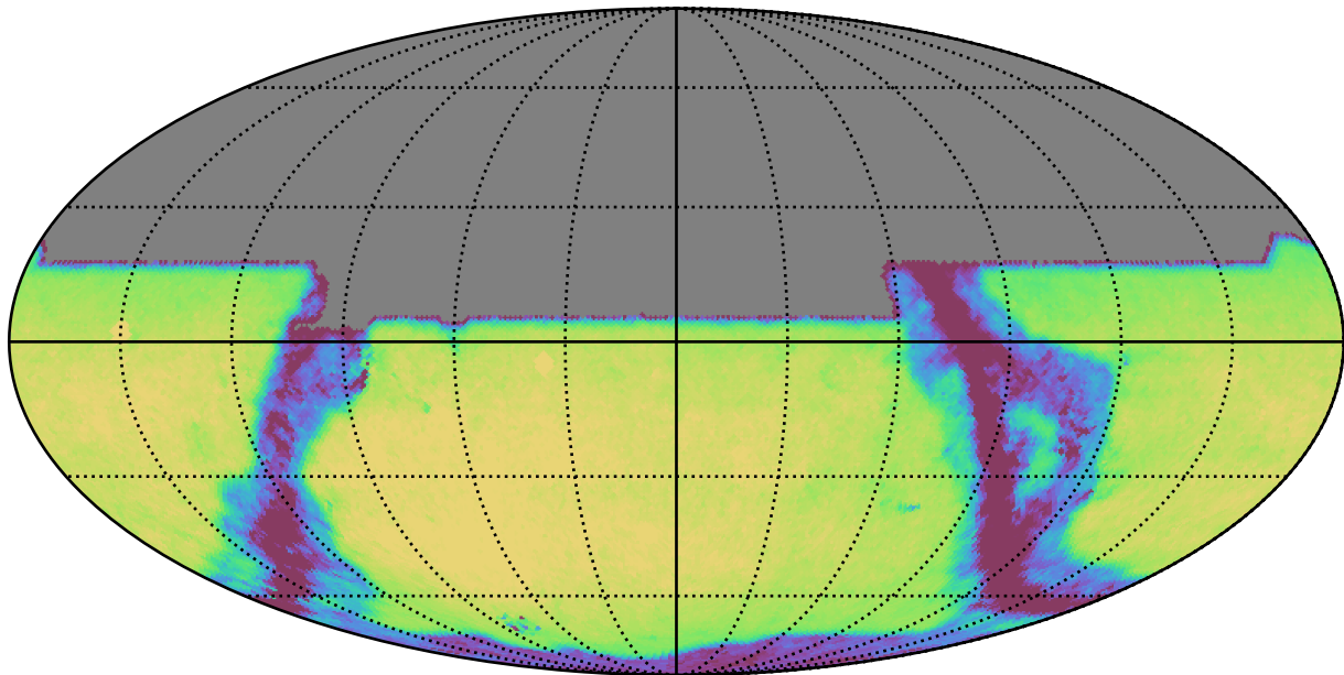
mw_roll_bulge_v3.3_10yrs All sky y band: Exgal_CoaddM5
