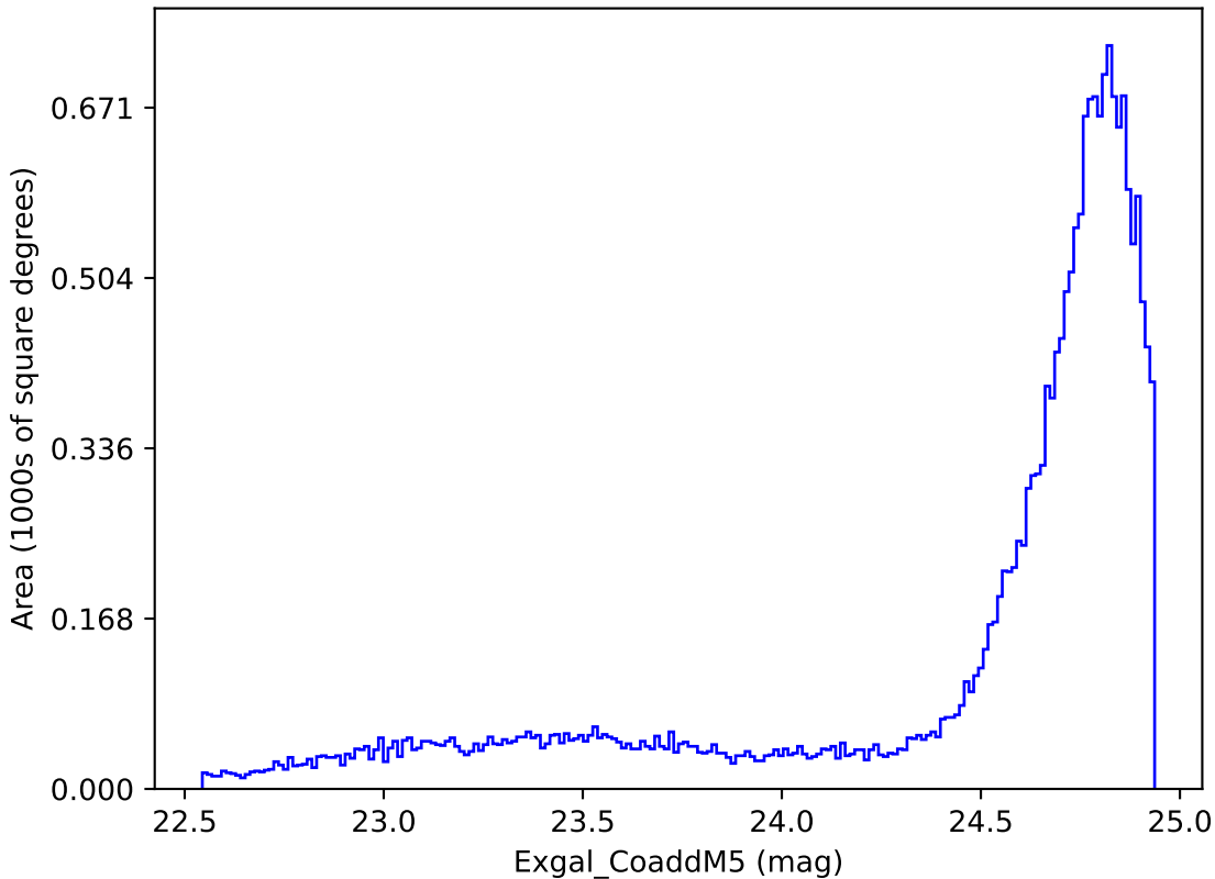
mw_roll_bulge_v3.3_10yrs All sky y band: Exgal_CoaddM5
