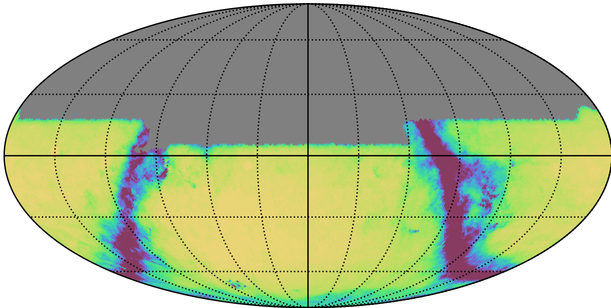
mw_roll_bulge_v3.3_10yrs All sky u band: Exgal_CoaddM5
