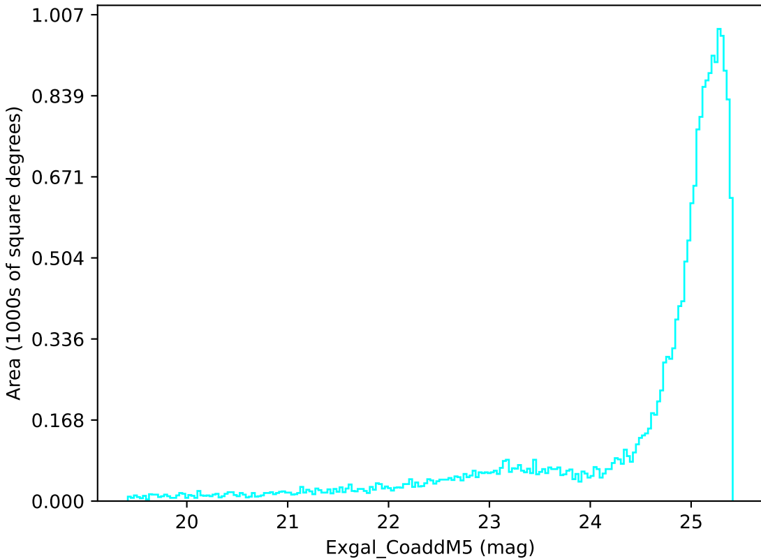
mw_roll_bulge_v3.3_10yrs All sky u band: Exgal_CoaddM5
