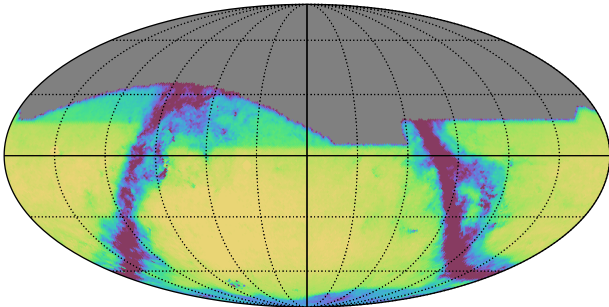
mw_roll_bulge_v3.3_10yrs All sky r band: Exgal_CoaddM5
