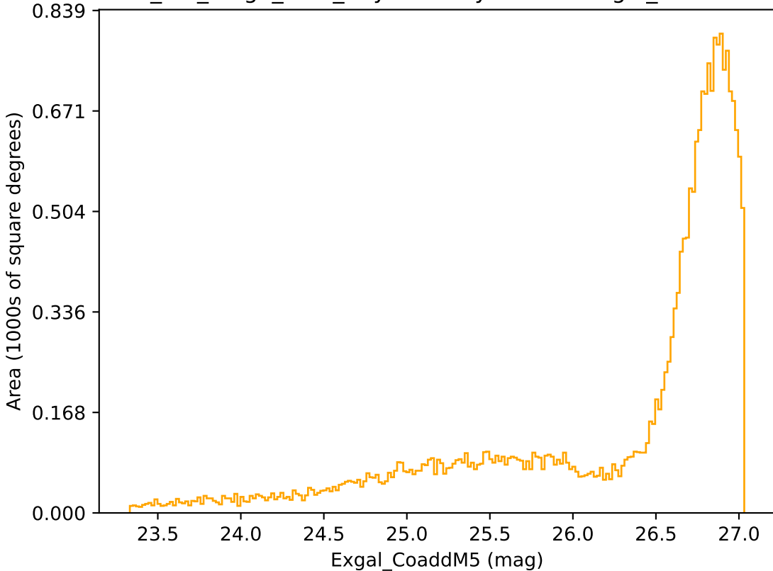
mw_roll_bulge_v3.3_10yrs All sky r band: Exgal_CoaddM5
