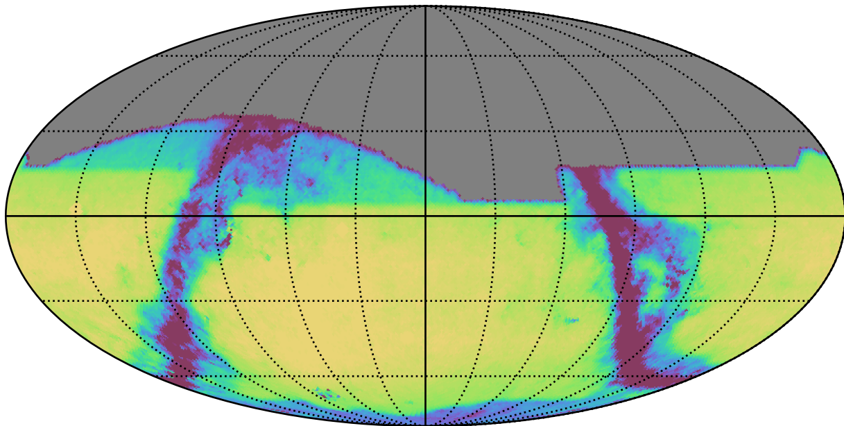
mw_roll_bulge_v3.3_10yrs All sky i band: Exgal_CoaddM5
