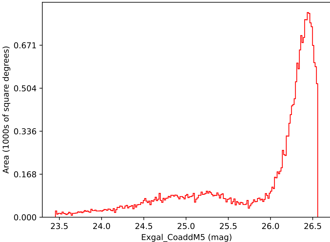
mw_roll_bulge_v3.3_10yrs All sky i band: Exgal_CoaddM5
