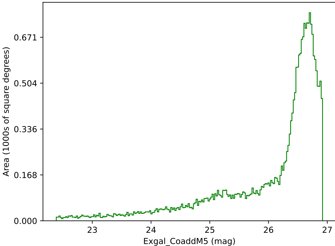
mw_roll_bulge_v3.3_10yrs All sky g band: Exgal_CoaddM5
