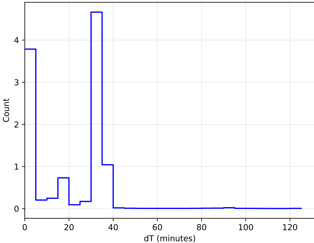
1e6 mw_roll_bulge_v3.3_10yrs WFD: DeltaT Histogram
