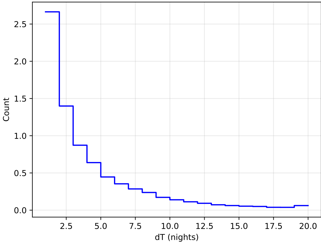
mw_roll_bulge_v3.3_10yrs WFD all bands: DeltaNight Histogram 1e6
