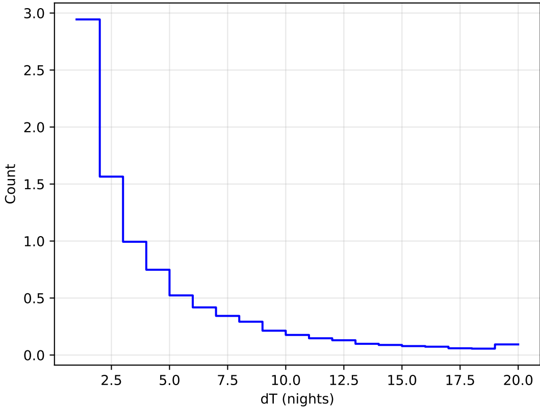
mw_roll_bulge_v3.3_10yrs All sky all bands: DeltaNight Histogram 1e6
