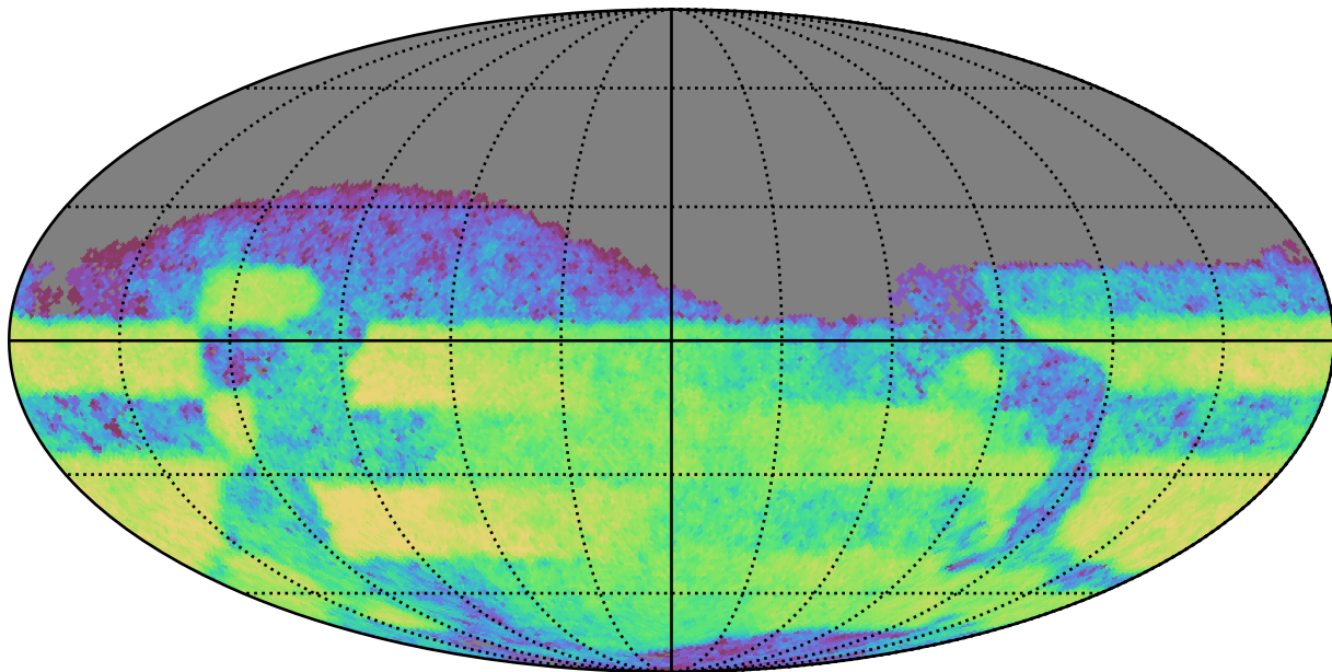
mw_roll_bulge_v3.3_10yrs Yr 3-4 z band: CoaddM5
