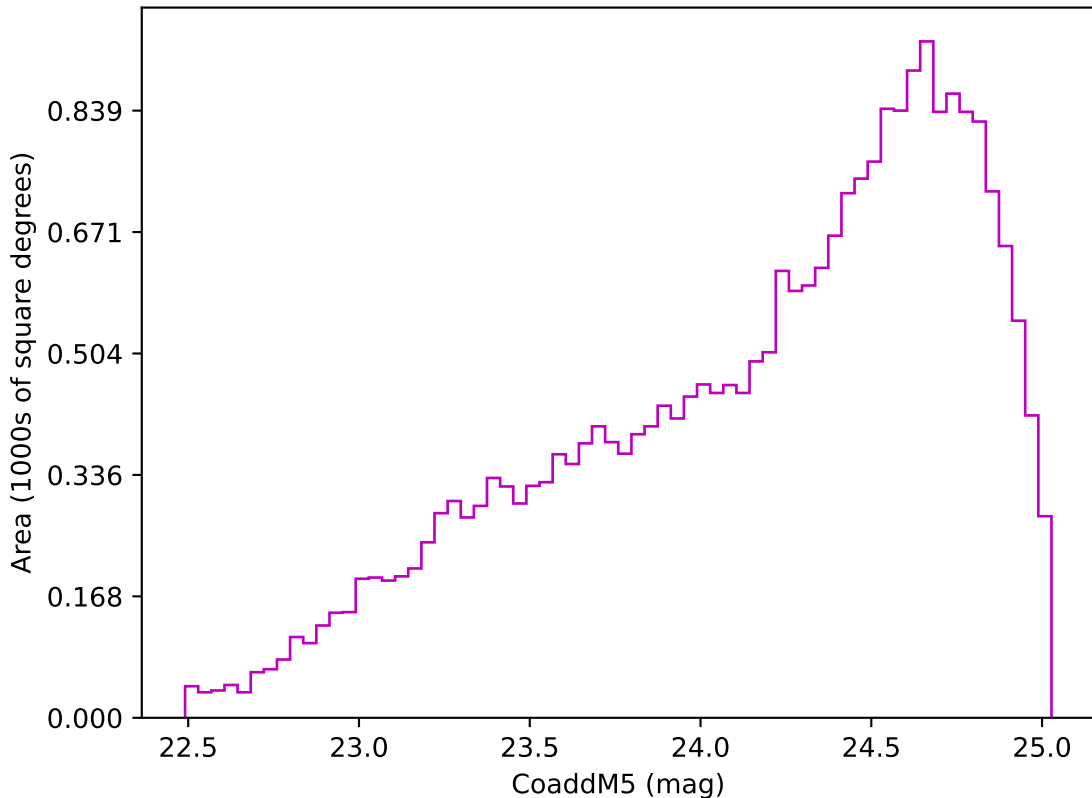
mw_roll_bulge_v3.3_10yrs Yr 3-4 z band: CoaddM5
