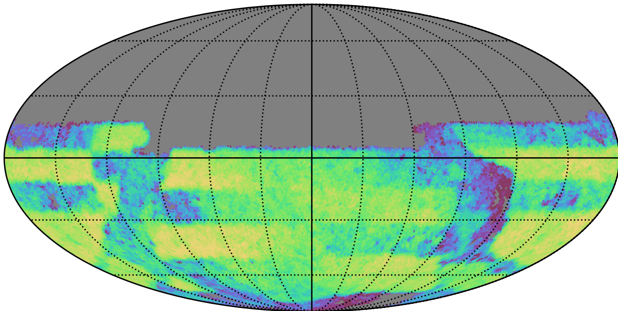
mw_roll_bulge_v3.3_10yrs Yr 3-4 y band: CoaddM5
