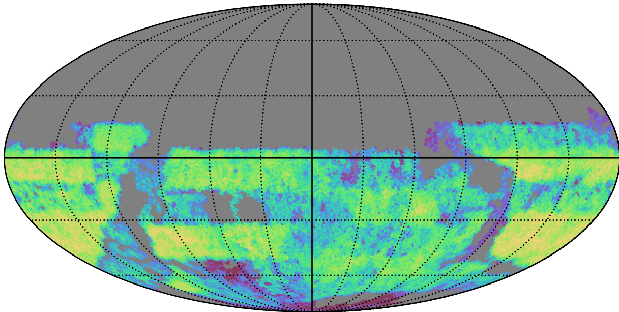
mw_roll_bulge_v3.3_10yrs Yr 3-4 u band: CoaddM5
