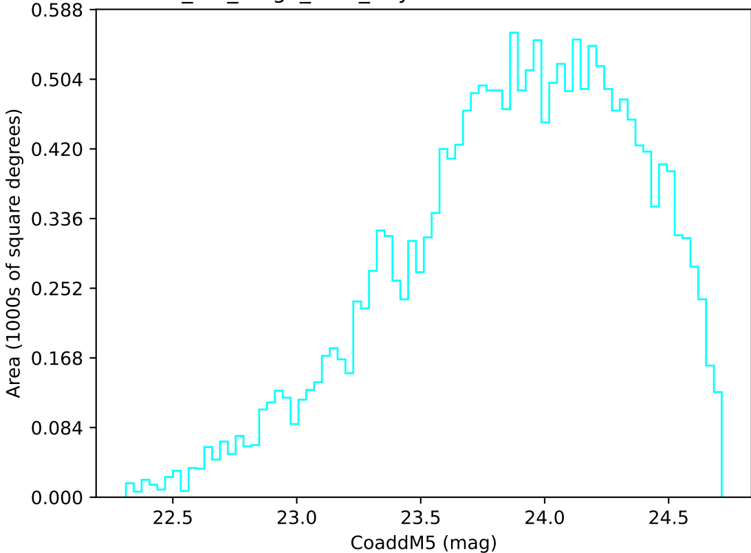
mw_roll_bulge_v3.3_10yrs Yr 3-4 u band: CoaddM5
