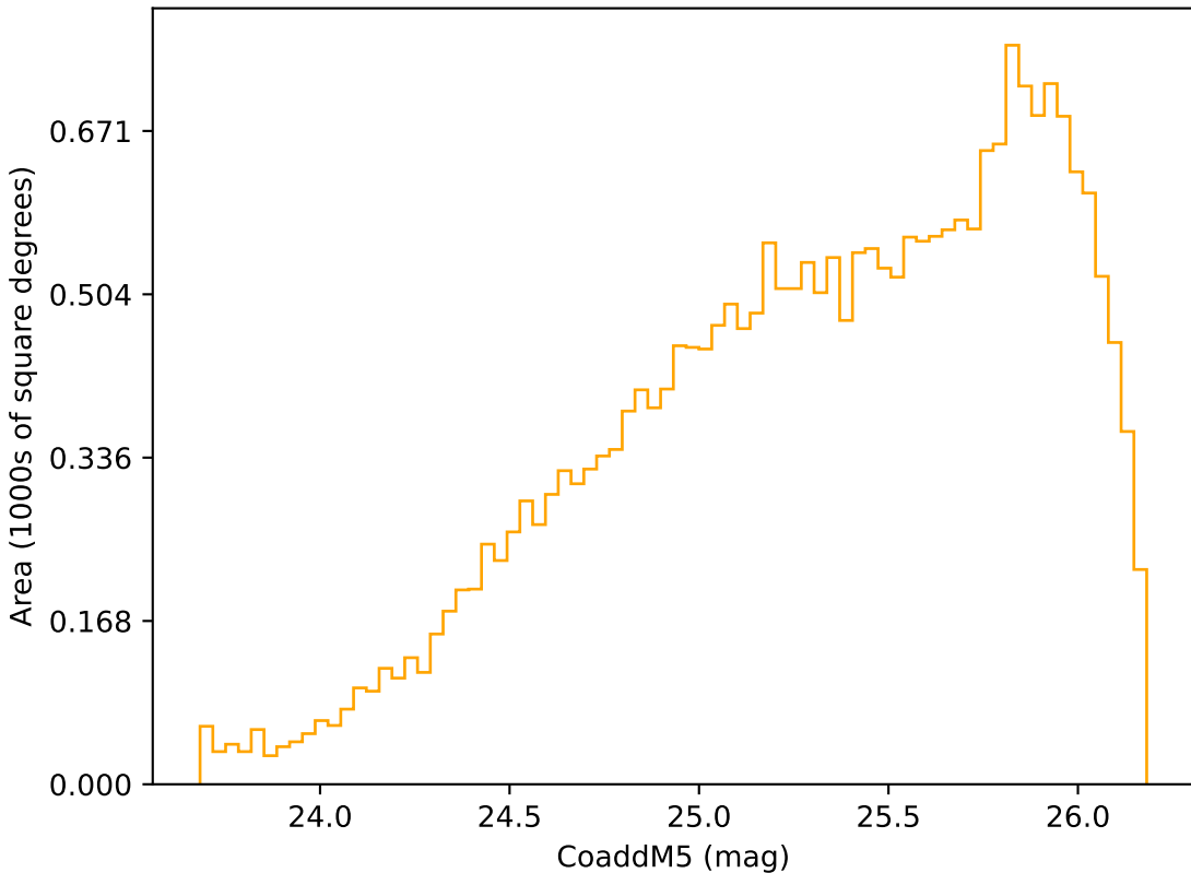
mw_roll_bulge_v3.3_10yrs Yr 3-4 r band: CoaddM5
