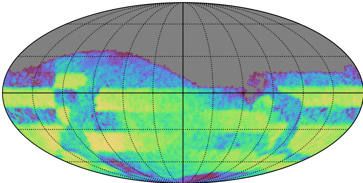
mw_roll_bulge_v3.3_10yrs Yr 3-4 i band: CoaddM5
