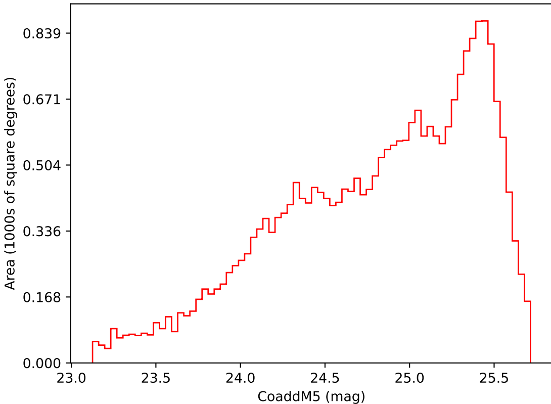
mw_roll_bulge_v3.3_10yrs Yr 3-4 i band: CoaddM5
