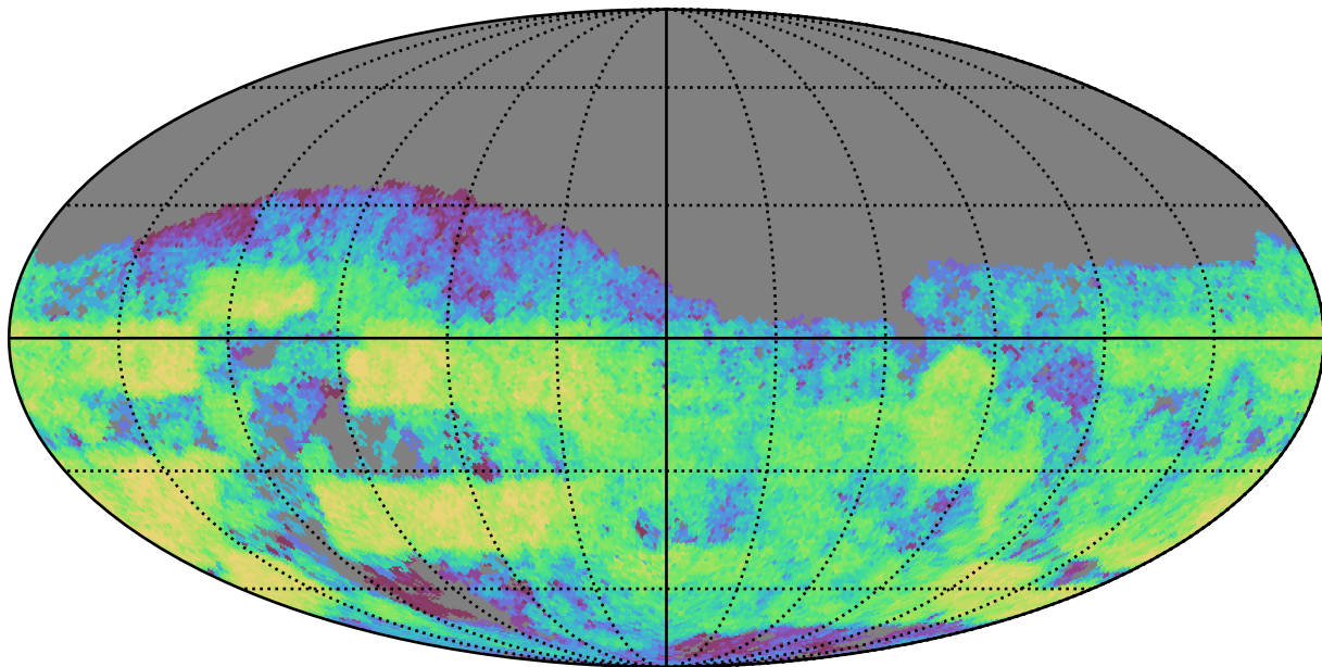
mw_roll_bulge_v3.3_10yrs Yr 3-4 g band: CoaddM5
