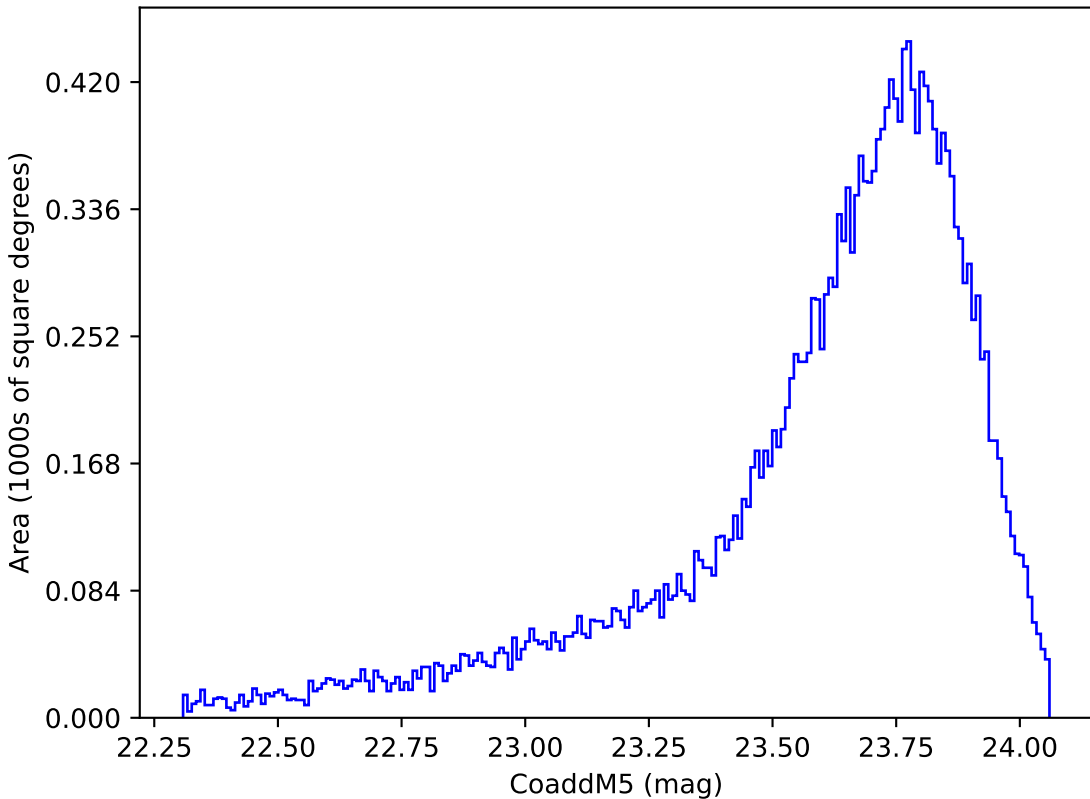
mw_roll_bulge_v3.3_10yrs Yr 1 y band: CoaddM5
