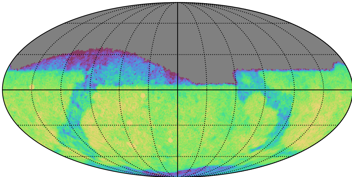
mw_roll_bulge_v3.3_10yrs Yr 1 r band: CoaddM5
