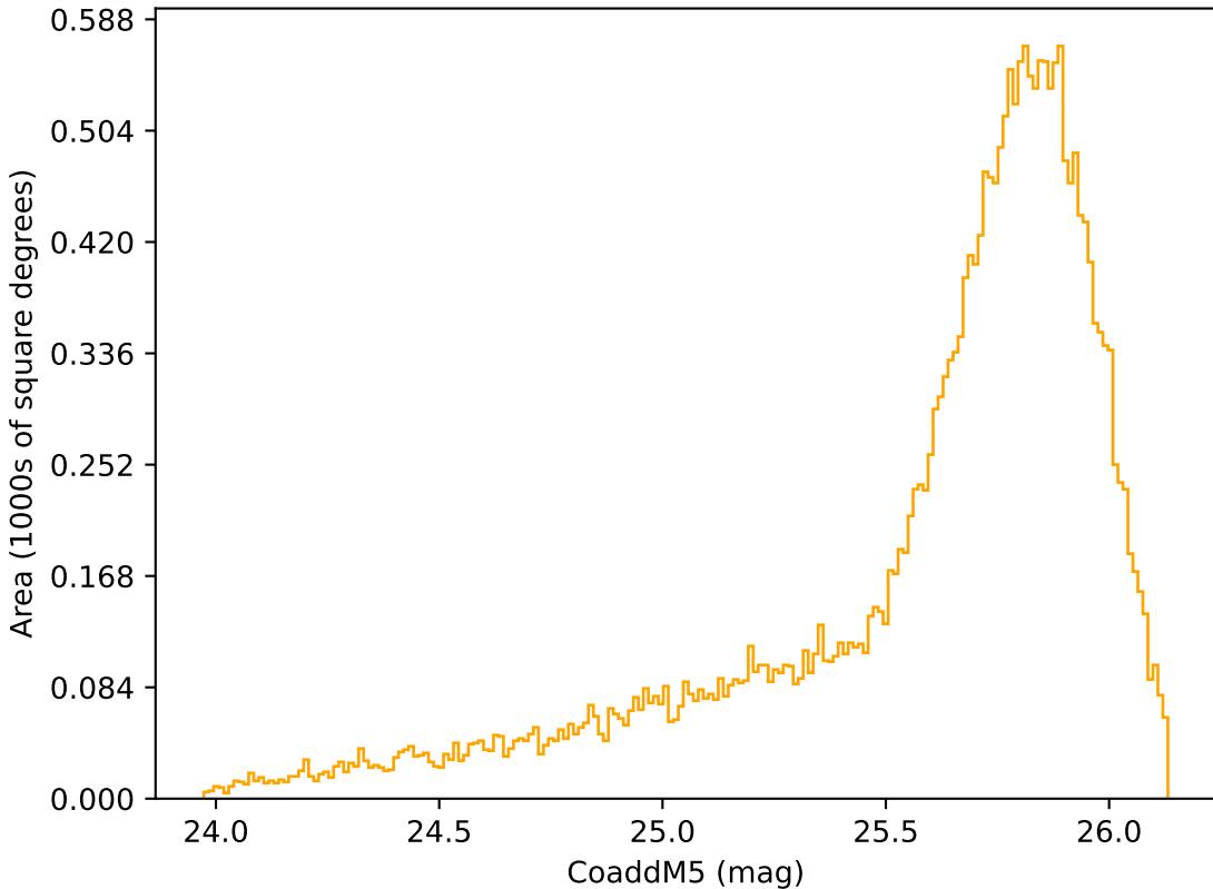
mw_roll_bulge_v3.3_10yrs Yr 1 r band: CoaddM5
