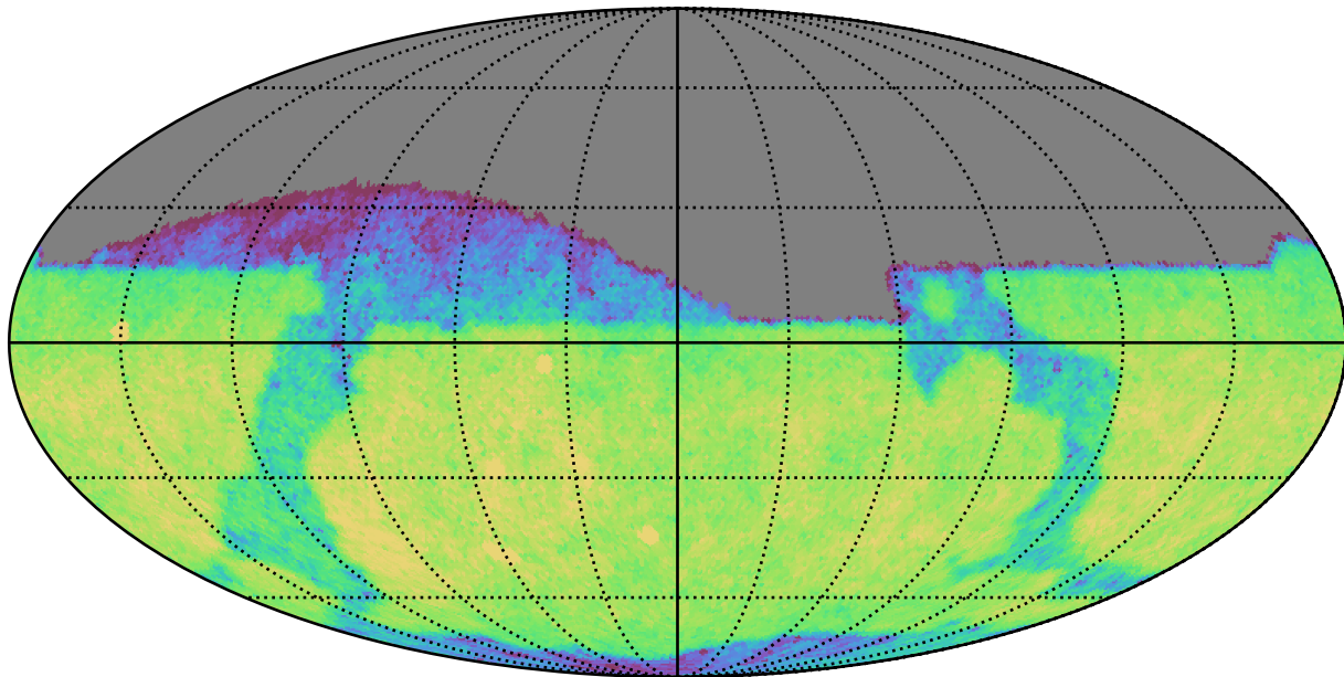
mw_roll_bulge_v3.3_10yrs Yr 1 i band: CoaddM5
