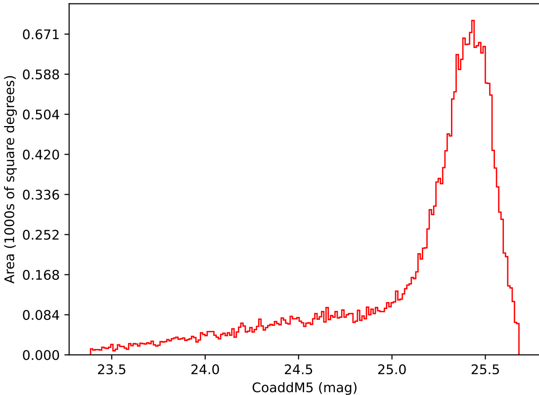
mw_roll_bulge_v3.3_10yrs Yr 1 i band: CoaddM5
