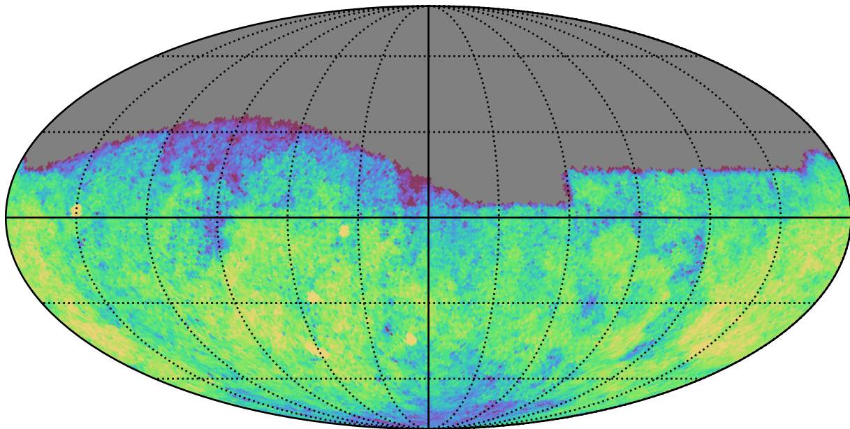
mw_roll_bulge_v3.3_10yrs Yr 1 g band: CoaddM5
