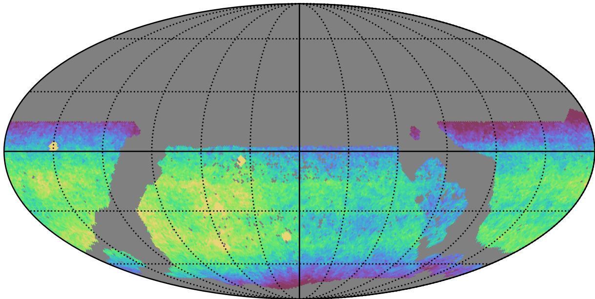
mw_roll_bulge_v3.3_10yrs WFD z band: CoaddM5
