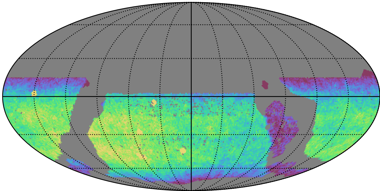
mw_roll_bulge_v3.3_10yrs WFD y band: CoaddM5
