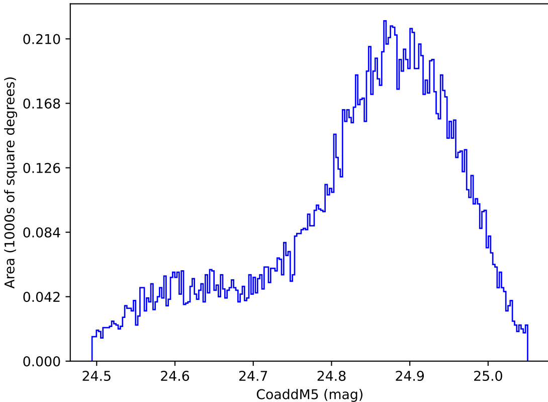
mw_roll_bulge_v3.3_10yrs WFD y band: CoaddM5
